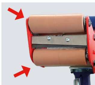
Double Contact Pressure Rollers
